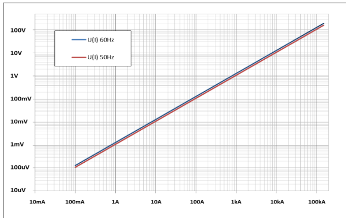
Characteristic of the U output voltage dependence on the current I
