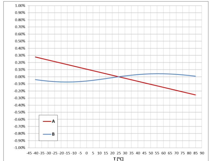
Characteristic of the dependence of the measurement error on temperature for R_o=47k\Omega (A - CR 1-25, B - CR 1-25-T)
