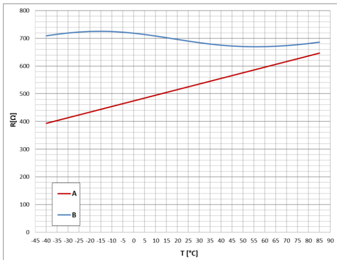
Characteristics of dependence of resistance on temperature (A - CR 1-25, B - CR 1-25-T)
