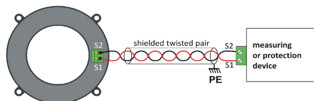
Connection diagram of the CR transformer
