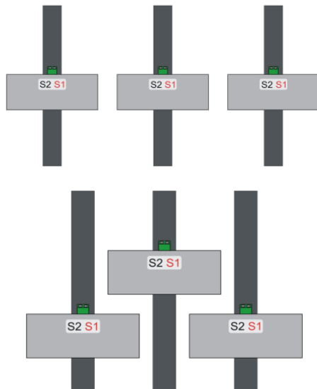
Correct mutual positioning of current transformers
