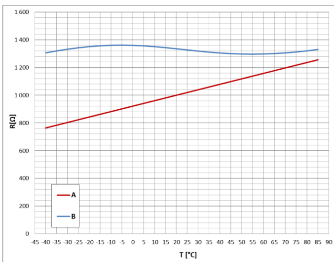
Characteristics of dependence of resistance on temperature (A - CRR 1-80, B - CRR 1-80-T)
