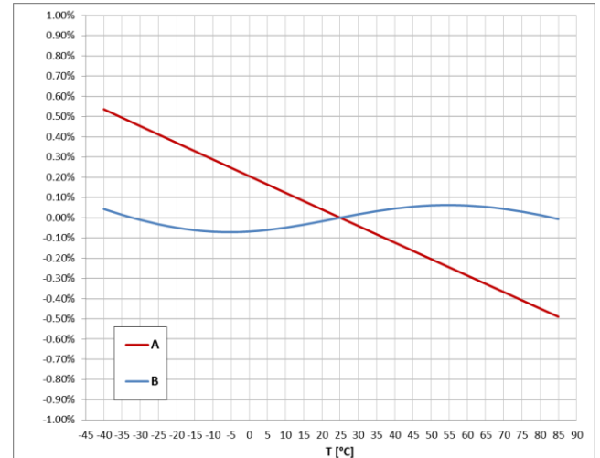
Characteristic of the dependence of the measurement error on temperature for R_o=47k\Omega (A - CRR 1-80, B - CRR 1-80-T)
