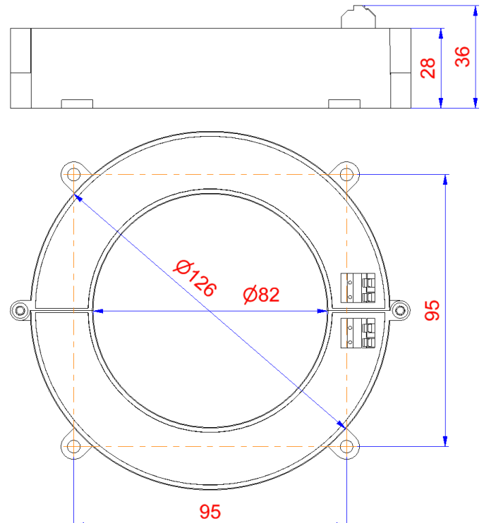
CRR 1-80, CRR 1-80-T housing
