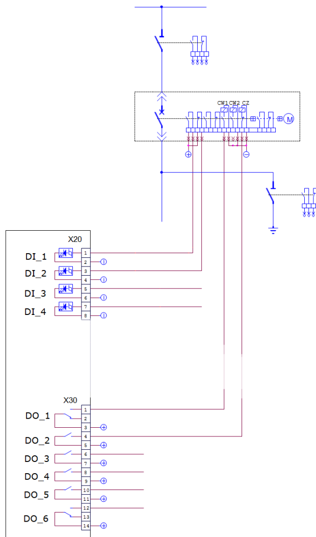
Fig. 5.1.2 State control and breaker control signals
