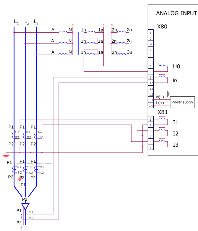
Fig. 5.1.1 Current and voltage transducer connection
