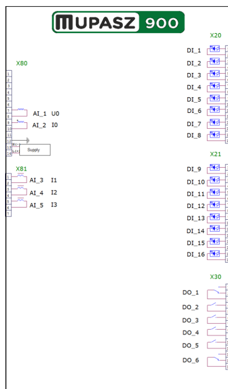
Fig. 5.2 Socket assignment example (8 binary inputs version)
